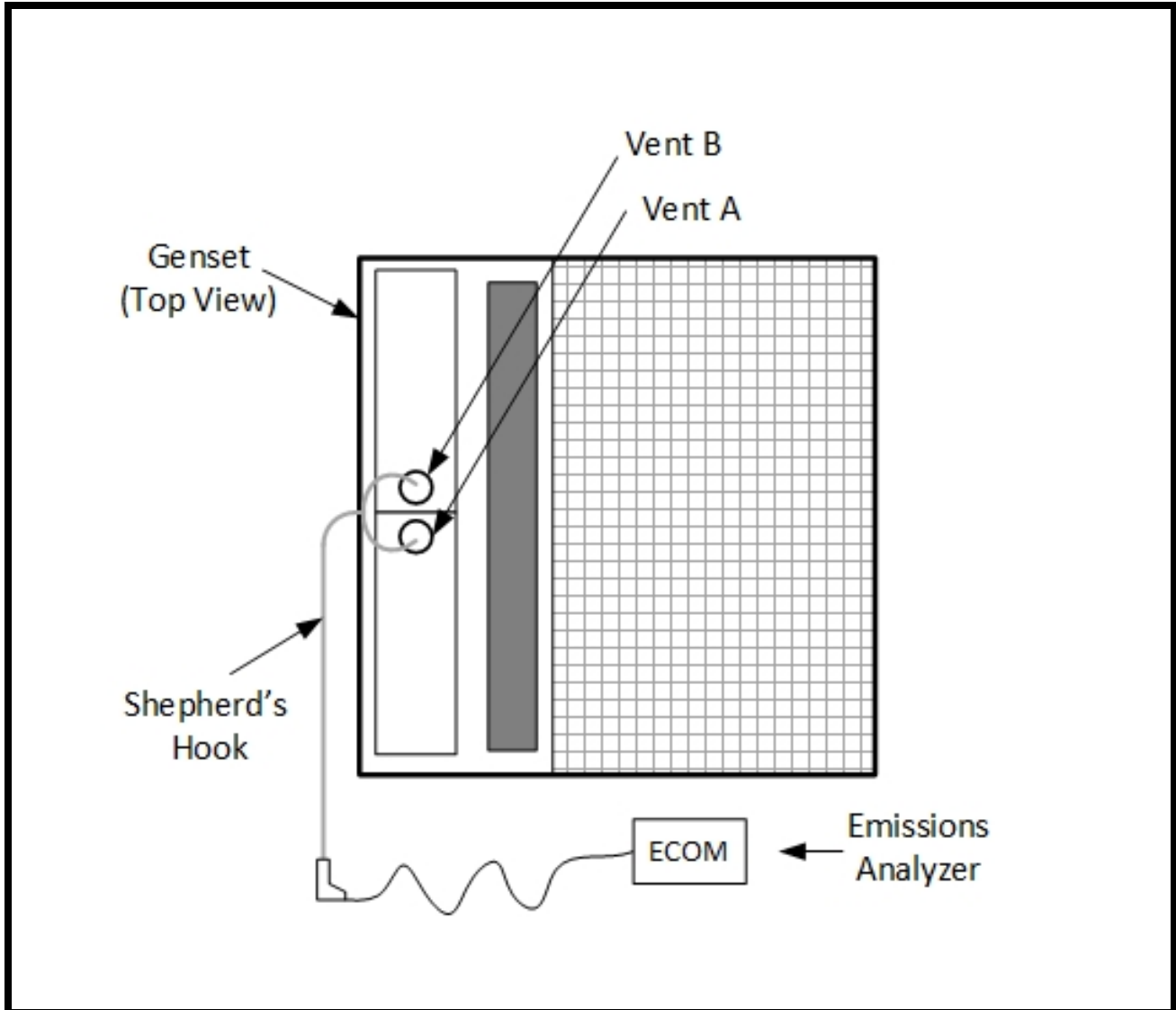
Figure 1-2 Emission Test Diagram
